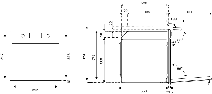
Cabinet Measures W 560-570, H 580-585, D 565-580
