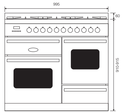
Front 60/40 split ovens
